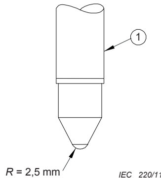
Figure 20 – Ball thrust tester
