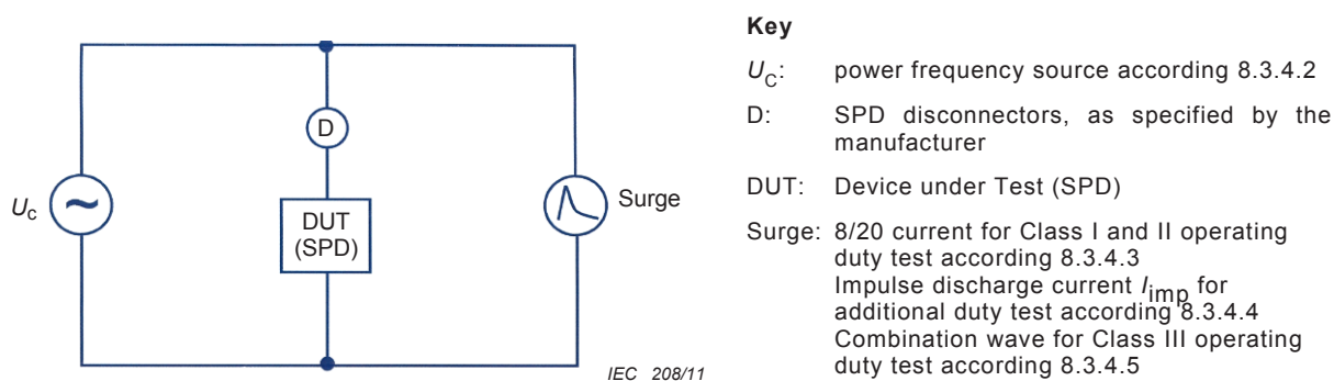
Figure 7 – Test set-up for operating duty test
